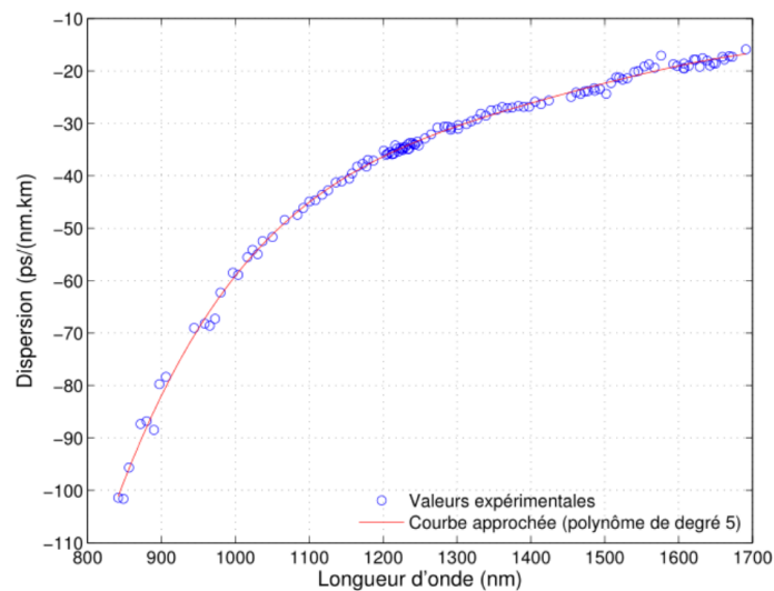
Chromatic Dispersion Polynomial fit (minimum 5 th order) at 1560nm
