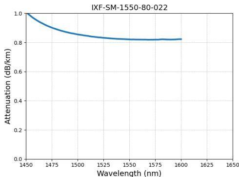
Typical attenuation spectrum of the IXF-SM-1550-80-022 fiber.
