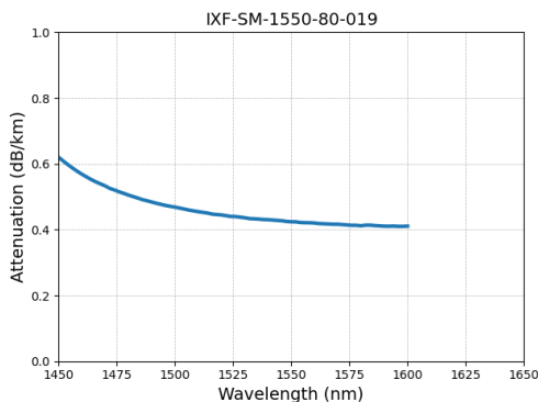
Typical attenuation spectrum of the IXF-SM-1550-80-019 fiber.
