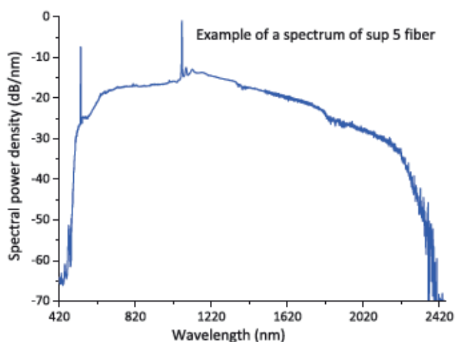
Typical supercontinuum generated in 10m of IXF-SUP-5-125-1050 with 300 mW 1064 nm pulse laser (1.2 ns @ 25 kHz)
