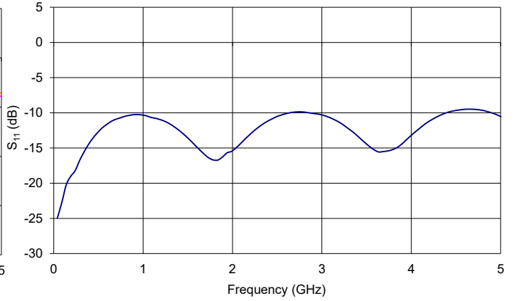
MX2000-LN-01 Typical S_{11} Curve
