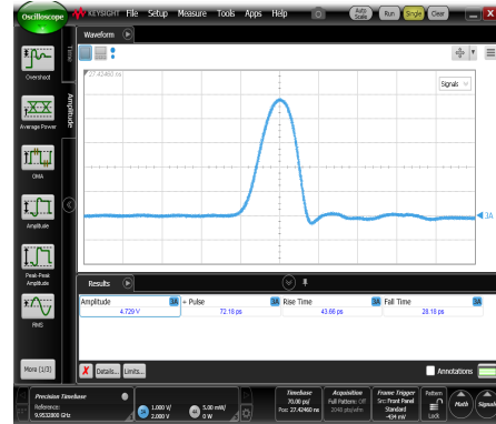
Output response: Pulse amplitude = 4.7 V pp , Rise time
