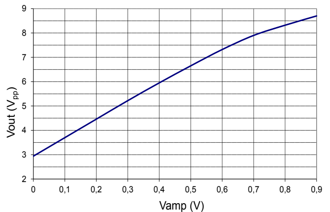
Typical Output Voltage Amplitude vs V_{amp}
