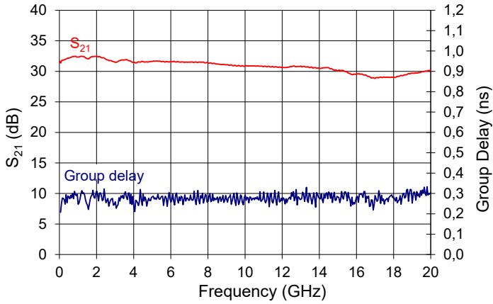
S_{21} and Group Delay Parameter Curves
