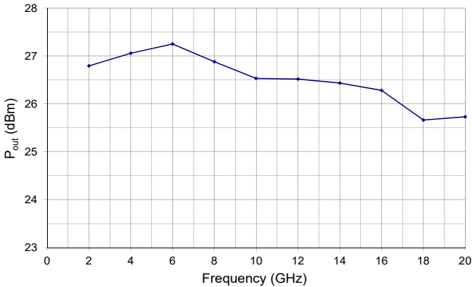
P_{out} @ 1dB Compression Curve
