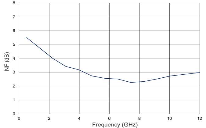
Noise Figure Curve
