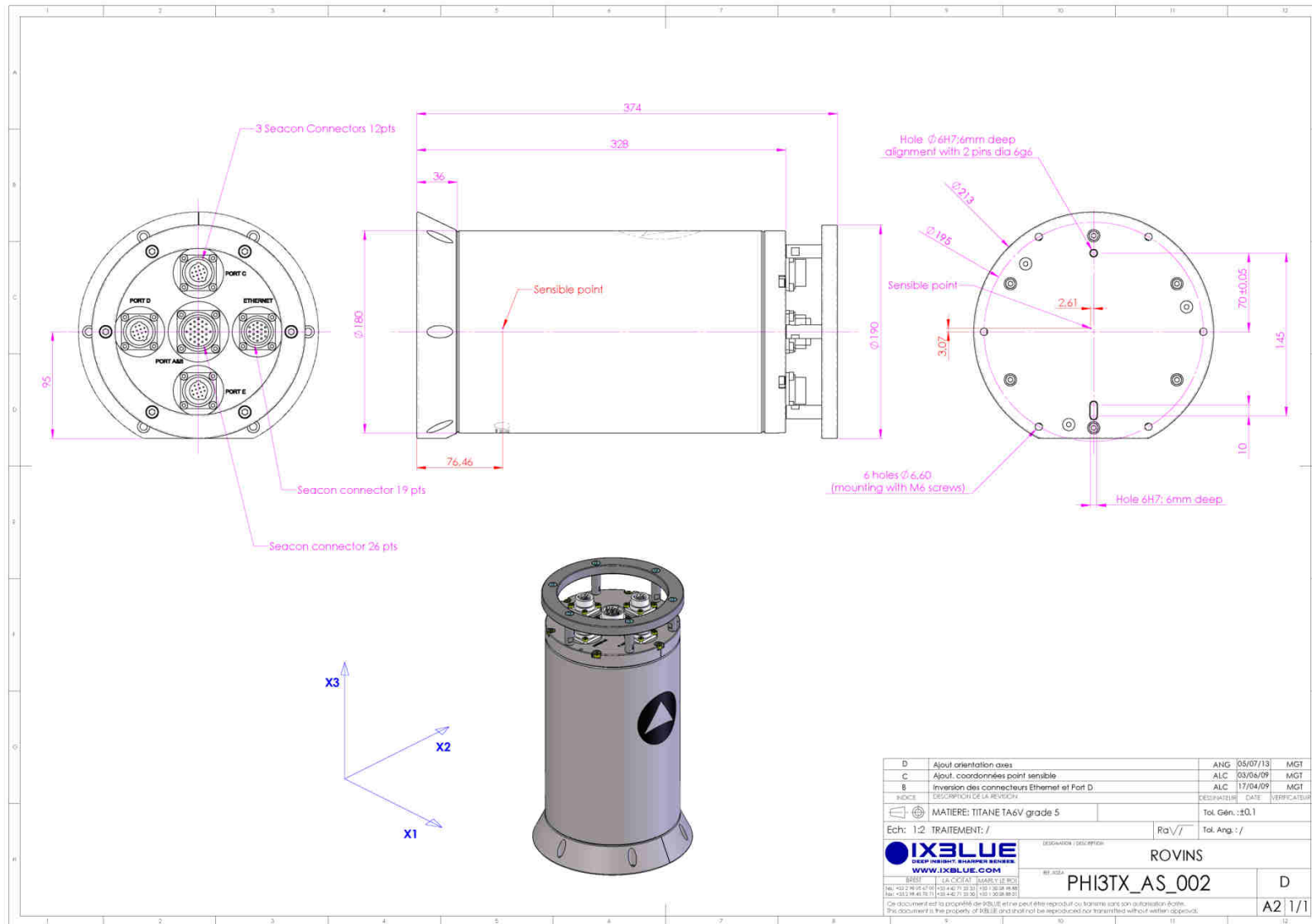
Figure 1 - ROVINS housing dimensions and sensitive point P
