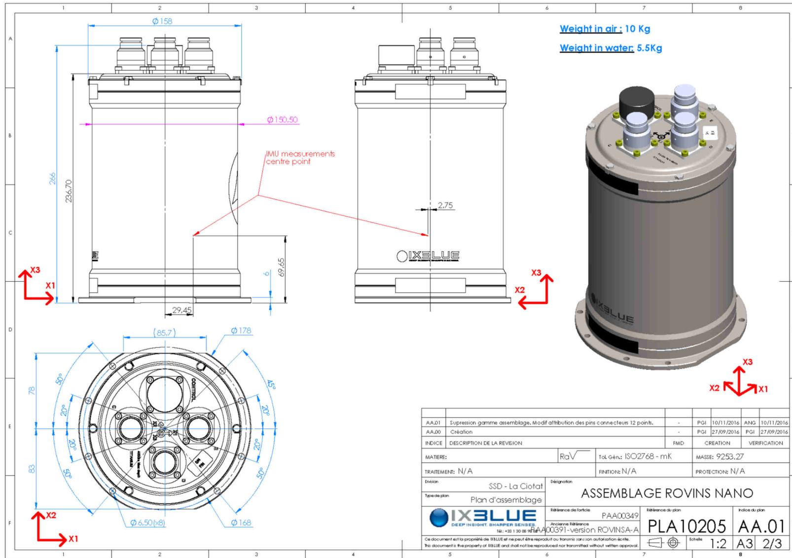
Figure 1 - ROVINS NANO housing dimensions and sensitive point P
