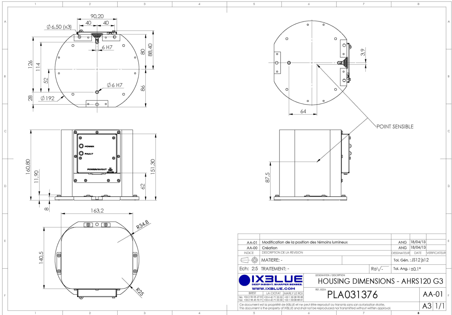
Figure 2 - Phins Compact C7 housing dimensions and centre point P
