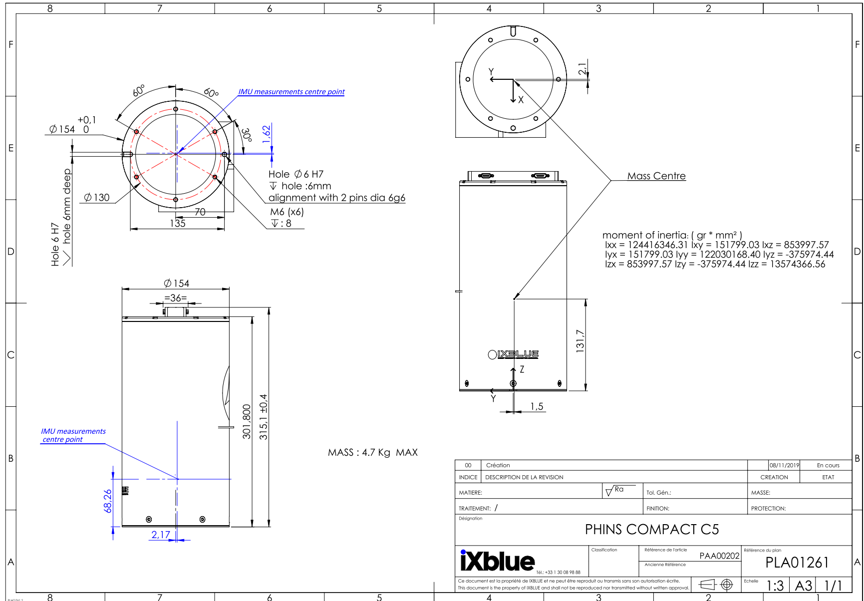
Figure 3 - Phins Compact C5 housing dimensions and centre point P
