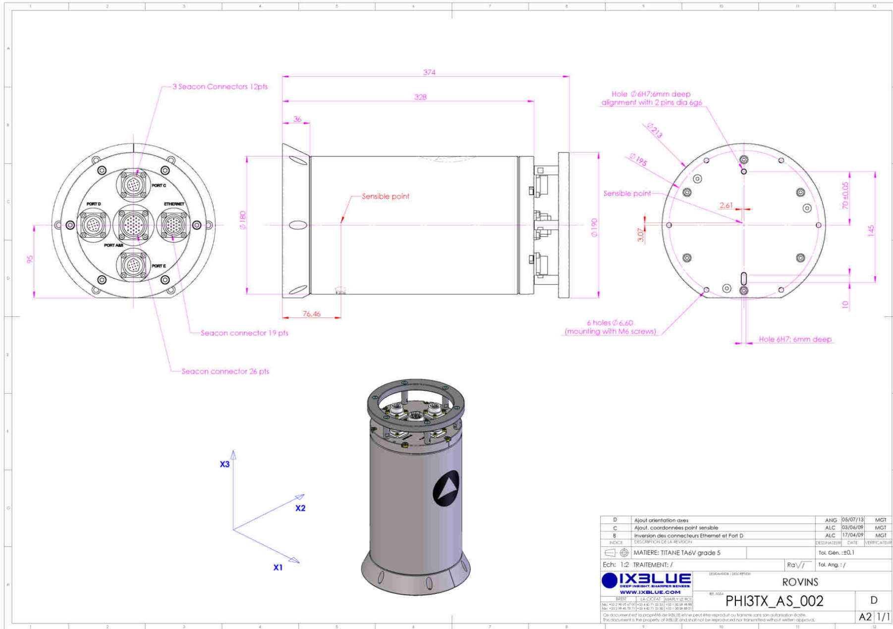
Figure 1 - OCTANS SUBSEA housing dimensions and sensitive point P
