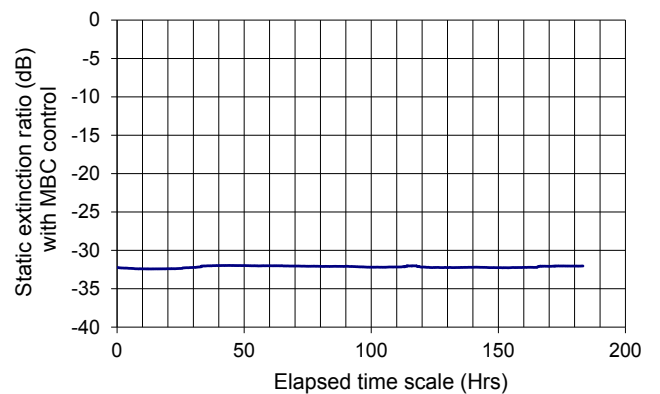
Stability with Time and Temperature
