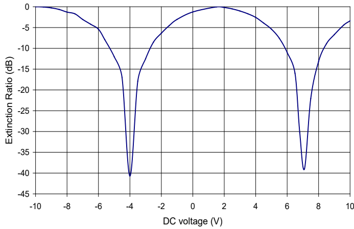
Extinction Ratio
