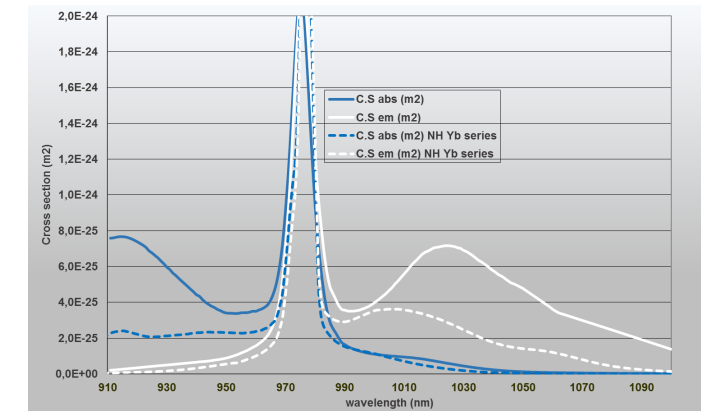
Yb Double Clad Cross section files
